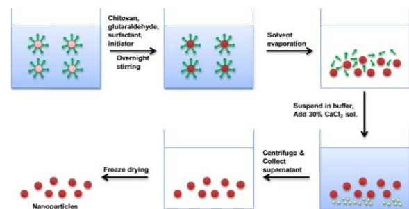
Fig. 2: Schematic representation of Micro emulsion method [8]
